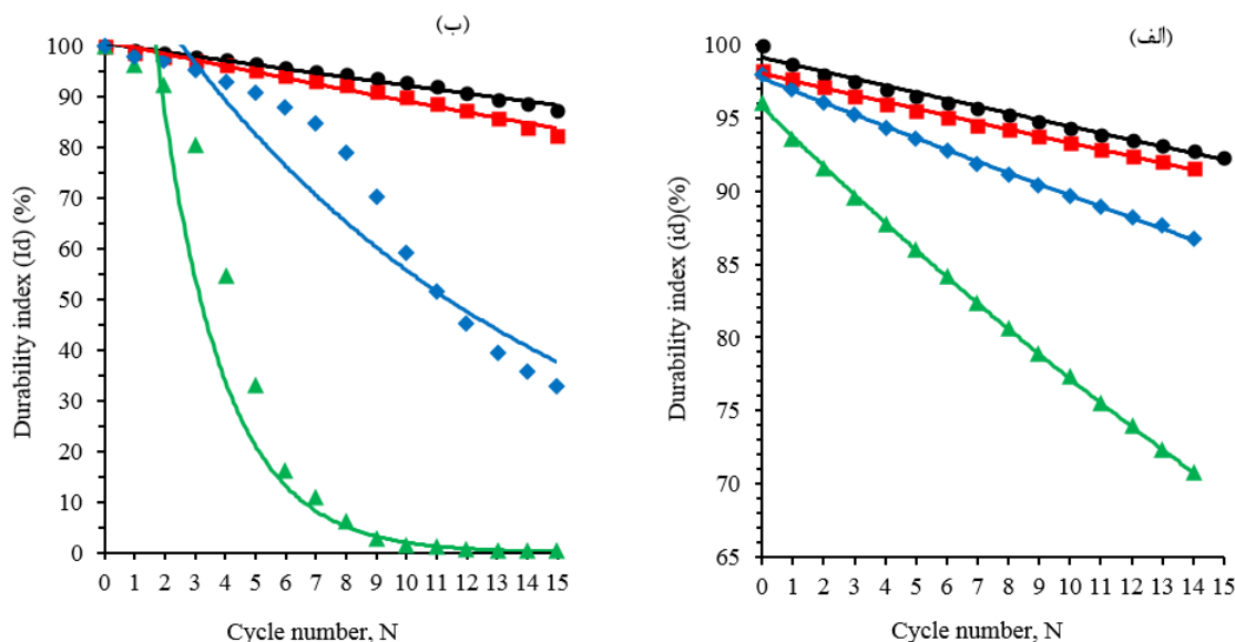
Fig. 6. Degradation constant diagram of the studied rock samples in the slake-durability test in a) normal water, and b) sodium sulfate solution
