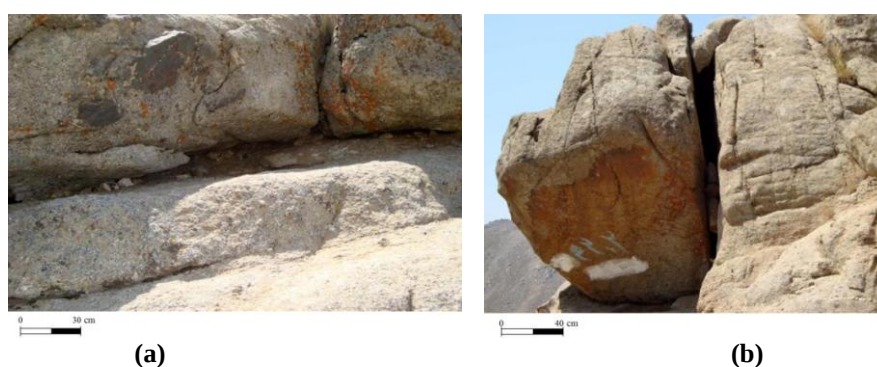
Figure2. Caves developed along a) horizontal, b) vertical fractures and joints
